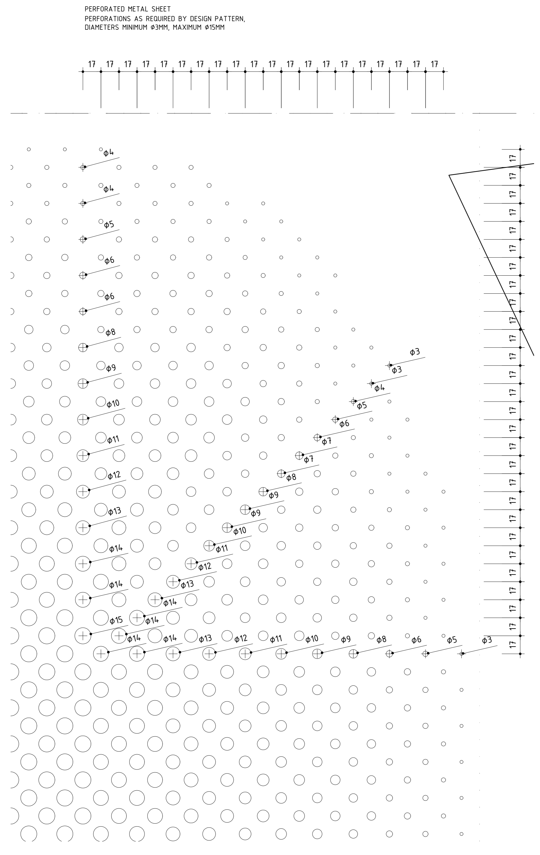
04 PERFORATED PANEL - HOLES DETAIL SCALE 1:2
